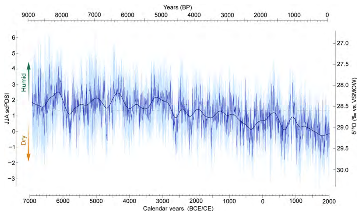
Fig. 4. Alpine summer hydroclimate reconstruction. Our \delta^{18}\text{O} TRSI-based JJA scPDSI reconstruction from the European Alps that covers the past 9000 years at a 5-year resolution (dark blue), together with its 500-year low-pass filter (smoothed line) and uncertainty range (light blue). The dashed horizontal line refers to the reconstructed long-term mean. VSMOW, Vienna Standard Mean Ocean Water.
