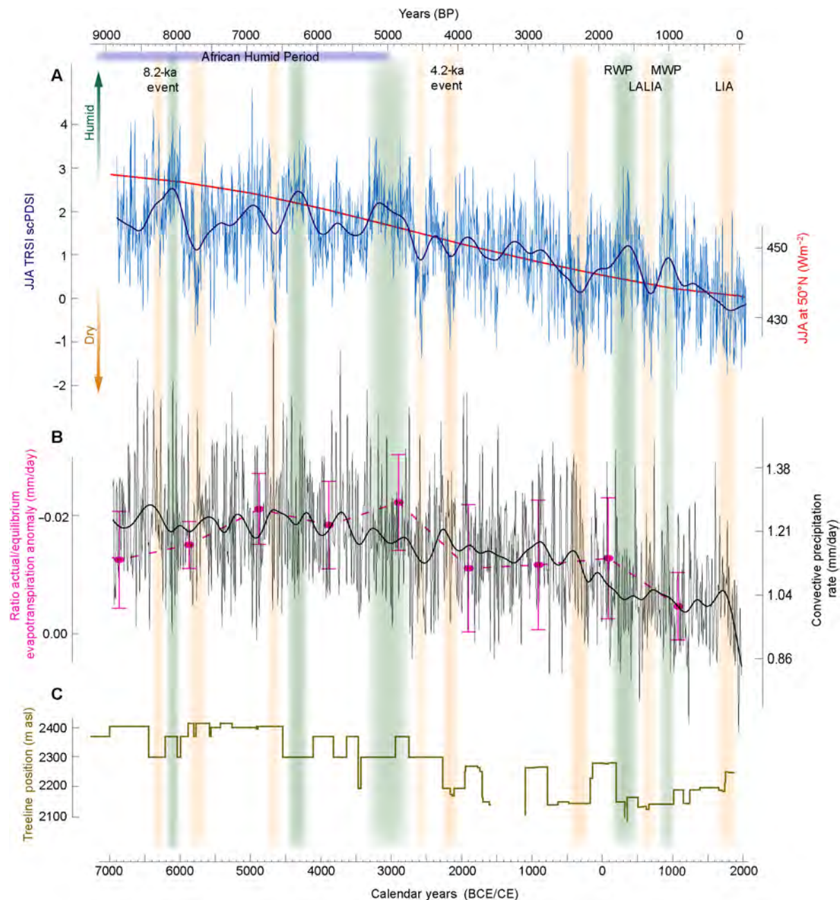
Fig. 5. Alpine climate and environmental changes over the Holocene. At the top, climatological phases shown are characteristic of the past 9000 years in central Europe and the Alpine arc, including the African Humid Period, the 8.2- and 4.2-ka events, the Roman Warm Period (RWP), the Medieval Warm Period (MWP), the Late Antique LIA (LALIA), and the LIA. (A) Our \delta^{18}\text{O} TRSI-based JJA scPDSI reconstruction from the European Alps (dark blue) and its 500-year low-pass filter (smoothed line), together with the accumulated Holocene orbital forcing for JJA at the mid-northern latitudes ( 50^\circ\text{N} ) (78, 79) (red line). Vertical bars highlight wet (light green) and dry (light red) episodes that deviate from the long-term trend of our reconstruction. (B) Mean annual ratio of the equilibrium evapotranspiration anomaly (in millimeters per day) reconstructed for the Holocene (pink) for the grid 46^\circ to 47^\circ\text{N} and 7.55^\circ to 12.25^\circ\text{E} (76). Annual mean value of the convective precipitation (black) simulated with the fully forced TraCE-21K for the grid 46^\circ to 47^\circ\text{N} and 7.55^\circ to 12.25^\circ\text{E} (77). (C) Estimated changes in the position of the upper treeline in the Austrian Alps (27). asl, above sea level.
