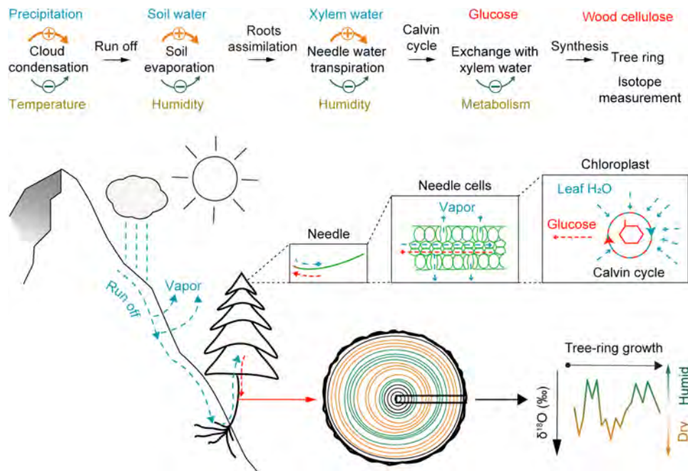
Fig. 2. Biotic and abiotic drivers of oxygen TRSIs. Oxygen isotopes ( \delta^{18}\text{O} ) in precipitation are subject to the Rayleigh distillation, where they are influenced by condensation temperature, whereas \delta^{18}\text{O} in soil water is influenced by evaporation, which is sensitive to humidity. The \delta^{18}\text{O} composition of leaf water is enriched by transpiration, which is mainly influenced by relative atmospheric humidity, and imprinted in the synthesis of glucose through the Calvin cycle under constant fractionation. Since glucose forms cellulose, tree-ring \delta^{18}\text{O} contains a distinct hydroclimate signal.
