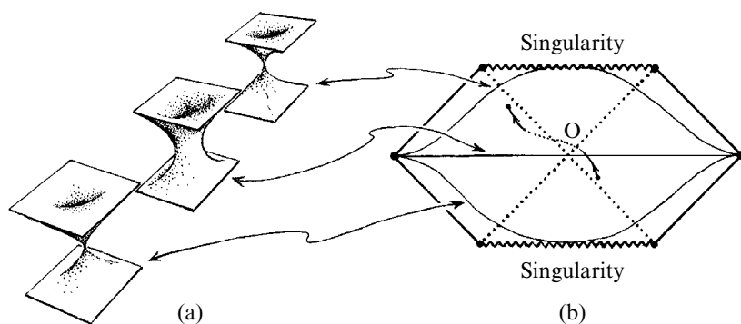
Fig. 30.8 The spacetime \mathcal{K} viewed globally as a ‘time-evolving’ 3-space, which represents a ‘wormhole’ connecting two asymptotically flat regions. The wormhole pinches off in a singular way, both into the future and into the past. Any space traveller who proposes to travel through the wormhole from one region to the other cannot get through before it ‘pinches off’ as is manifest from the conformal diagram, since this would demand the traveller’s worldline having a spacelike (superluminary) portion—shown dotted.
