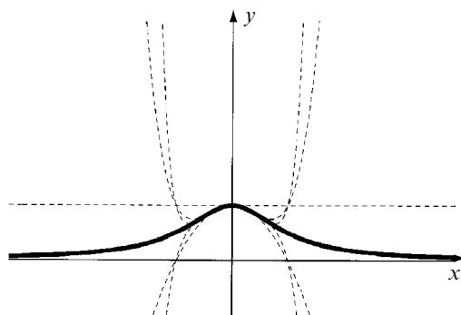
Fig. 4.2 The partial sums, 1, 1 - x^2, 1 - x^2 + x^4, 1 - x^2 + x^4 - x^6, 1 - x^2 + x^4 - x^6 + x^8 , of the series for (1 + x^2)^{-1} are likewise plotted, and again there is convergence for |x| < 1 and divergence for |x| > 1 , despite the fact that the function is perfectly well behaved at x = \pm 1 .
