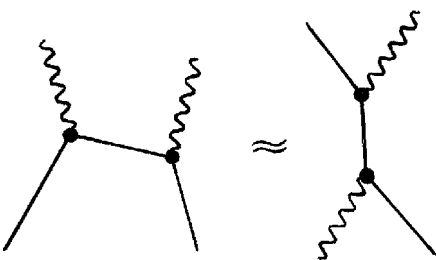
Fig. 25.10 Crossing symmetry. Processes which differ only with respect to the time-orderings in various places, but without the topology of the diagram being affected, are basically mathematically equivalent (through analytic continuation, §7.4). This is illustrated by such an equivalence between the particle–antiparticle pair annihilation into two photons, as illustrated on the left, and the Compton scattering process on the right (drawn without zigzags).
