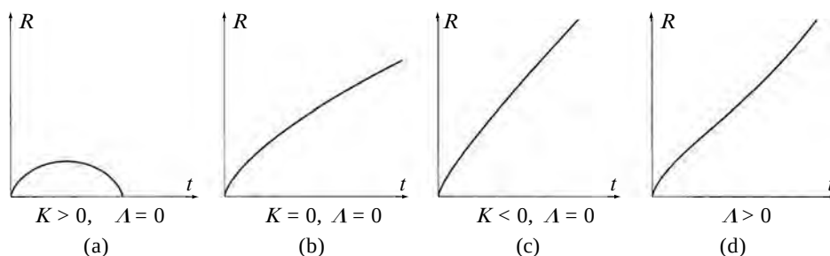
Fig. 27.15 Graphs of R = R(t) for Friedmann models, first with \Lambda = 0 : (a) K > 0 , (b) K = 0 , (c) K < 0 , and then (d) with \Lambda > 0 . (Case (d) is plotted for K = 0 , but the other cases are very similar, provided that \Lambda is large enough in relation to spatial curvature.)
