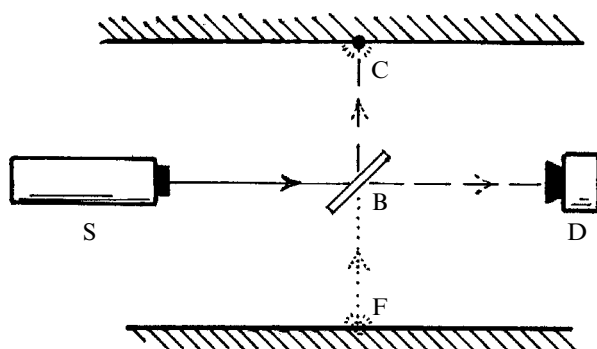
Fig. 30.1 A source S randomly emits single high-energy photons (each such event being recorded) aimed at a beam-splitter B, tilted at 45^\circ to the beam. If transmitted through B, the photon activates a detector D (route SBD); if reflected, it is absorbed at the ceiling C (route SBC). The quantum squared-modulus rule correctly predicts probabilities \frac{1}{2} , \frac{1}{2} . On the other hand, given that D registers, the photon could have come from S (route SBD) or from the floor F (route FBD). Used in the reversed-time direction, the squared-modulus rule incorrectly retrodicts probabilities \frac{1}{2} , \frac{1}{2} , which should be 1, 0.
