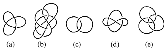
Fig. 32.6 Knots and links. (a) A trefoil knot—an example of a knotted loop. (b) An example of a (non-obviously, to the eye) un-knotted loop. (c) A simple link between two loops. (d) A Whitehead link, where the two loops cannot be separated though they have zero ‘linking number’ (the net number of times each meets a surface spanning the other) (e) Borromean rings, which cannot be separated, despite no pair of them being linked.
