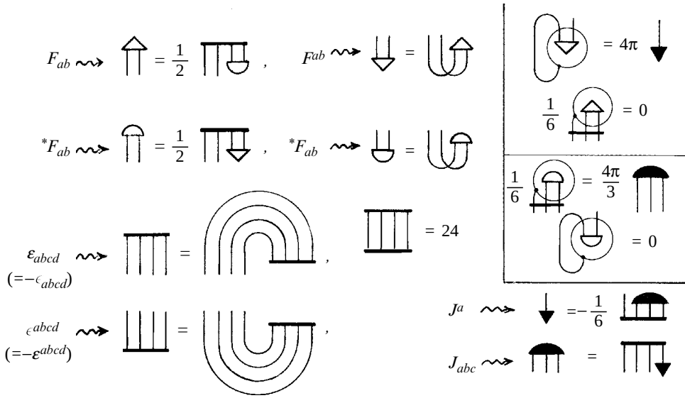
Fig. 19.1 Diagrams for Hodge duals and Maxwell equations. The quantities \varepsilon_{abcd} (= \varepsilon_{[abcd]}) and \epsilon^{abcd} (= \epsilon^{[abcd]}) , normalized so that \epsilon_{0123} = \epsilon^{0123} = 1 in a standard Minkowski frame, are related to their raised/lowered versions (via g^{ab} and g_{ab} ) by \varepsilon_{abcd} = -\epsilon_{abcd} and \epsilon^{abcd} = -\varepsilon^{abcd} . In the diagrams (left middle, lower two lines) this sign change is absorbed by an effective index reversal. Boxed off at the top right are the Maxwell equations, first using the field tensor F (with its raised form F^{ab} = g^{ac}g^{bd}F_{cd} ; cf. Fig. 14.21) so the equations are \nabla_a F^{ab} = 4\pi J^b , \nabla_{[a} F_{bc]} = 0 , and beneath that, correspondingly using the dual *F (where *F_{ab} = \frac{1}{2}\varepsilon_{abcd}F^{cd} , *J_{abc} = \varepsilon_{abcd}J^d ) so the equations are \nabla_{[a} *F_{bc]} = \frac{4\pi}{3} *J_{abc} , \nabla_a *F^{ab} = 0 .
