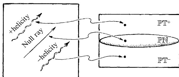
Fig. 33.6 The real 5-manifold \mathbb{PN} divides projective twistor space \mathbb{PT} into two complex-3-manifold pieces \mathbb{PT}^+ and \mathbb{PT}^- , these representing massless particles of positive and of negative helicity, respectively.
