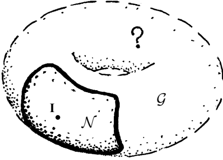
Fig. 13.12 The Lie algebra for a (faithful) representation of a Lie group \mathcal{G} (basically, knowledge of the structure constants \gamma_{\alpha\beta}^{\lambda} ) determines the local structure of \mathcal{G} , i.e. it fixes the structure of \mathcal{G} within some (sufficiently small) open region \mathcal{N} surrounding the identity element \mathbf{I} , but it does not tell us about the global nature of \mathcal{G} .
