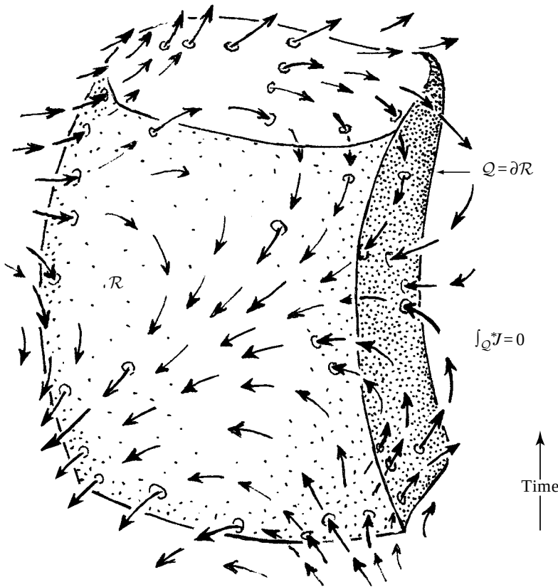
Fig. 19.3 Conservation of electric charge in spacetime. The closed 3-surface Q is the boundary Q = \partial\mathcal{R} of a compact 4-volume \mathcal{R} , in Minkowski spacetime \mathbb{M} , so the fundamental theorem of exterior calculus tells us \int_Q J = \int_{\mathcal{R}} d^*J = 0 , since d^*J = 0 . The quantity J describes the ‘flux’ (or ‘flow’) of charge across Q , so the total charge flowing in across Q is equal to that flowing out, expressing charge conservation.
