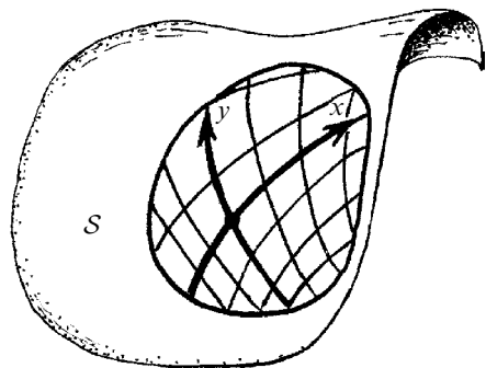
Fig. 10.3 Within one local patch, smooth (real-number) coordinates (x, y) label the points.
