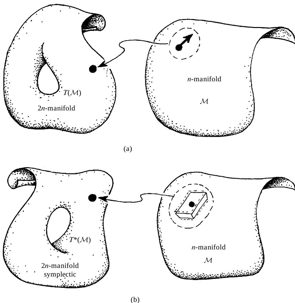
Fig. 15.12 (a) For a general manifold \mathcal{M} , each point of its tangent bundle T(\mathcal{M}) represents a point of \mathcal{M} together with a tangent vector to \mathcal{M} there. A cross-section of T(\mathcal{M}) represents a vector field on \mathcal{M} . (b) The cotangent bundle T^*(\mathcal{M}) is similar, but with covectors instead of vectors. Cotangent bundles are always symplectic manifolds.
