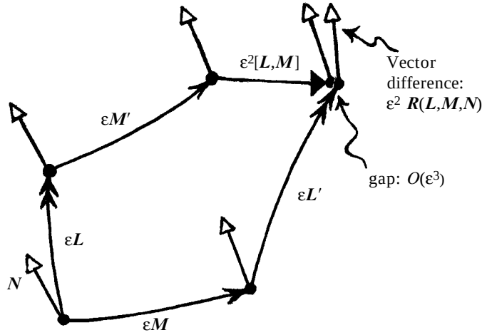
Fig. 14.19 Curvature, in the ‘mathematician’s notation’ (\nabla_L M - \nabla_M L - \nabla_{[M, L]} N = R(L, M, N) , from the O(\epsilon^2) discrepancy in parallel transport of a vector N around the (incomplete) ‘quadrilateral’ with sides \epsilon L , \epsilon M , \epsilon L' , \epsilon M' . The Lie bracket contribution \epsilon^2[L, M] fills an O(\epsilon^2) gap, to order O(\epsilon^3) . (The index form of the vector R(L, M, N) is L^a M^b N^c R_{abc}{}^d .)
