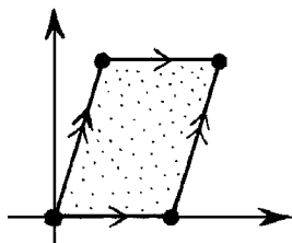
Fig. 8.10 To construct a Riemann surface of genus 1, take a region of the complex plane bounded by a parallelogram, vertices 0, 1, 1 + p , p (cyclicly), with opposite edges identified. The quantity p provides a modulus for the Riemann surface.
