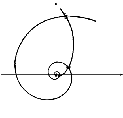
Fig. 5.9 The different values of w^z ( = e^{z \log w} ). Any integer multiple of 2\pi i can be added to \log z , which multiplies or divides w^z by e^{z \cdot 2\pi i} an integer number of times. In the general case, these are represented in the complex plane as the intersections of two equiangular spirals (each making a constant angle with straight lines through the origin).
