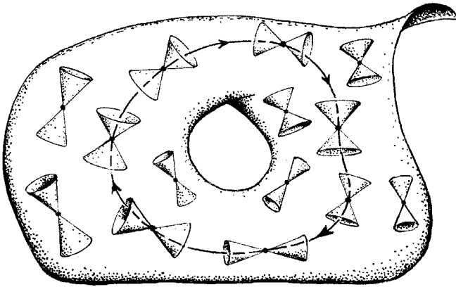
Fig. 17.18 The causality structure of \mathcal{E} is determined by g (as with \mathcal{M} , see Fig. 17.16), so extreme unphysical situations with ‘closed timelike curves’ might hypothetically arise, allowing future-directed signals to return from the past.
