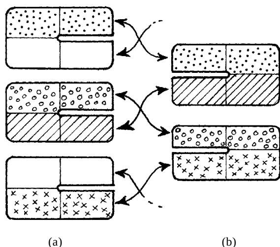
Fig. 8.3 We can construct the Riemann surface for \log z by taking alternate patches of (a) the complex plane with the non-negative real axis removed, and (b) the complex plane with the non-positive real axis removed. The top half each (a)-patch is glued to the top half of the next (b)-patch, and the bottom half of each (b)-patch glued to the bottom half of the next (a)-patch.
