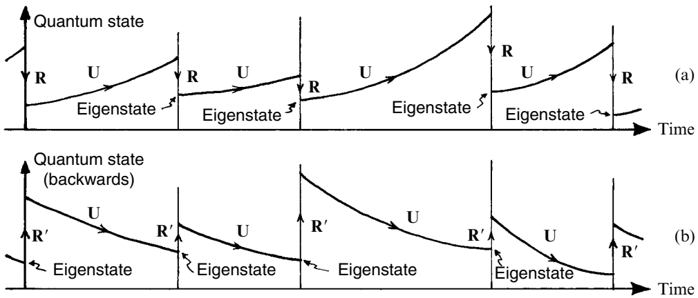
Fig. 30.2 Schematic illustration of the alternation... U, R, U, R, U, \dots of the two processes U and R as used in practice in quantum mechanics (compare Fig. 22.1), according to: (a) standard time-direction of evolution, where operator eigenstates occur at the past end of each stretch of U -evolution, and (b) time-reversed viewpoint of evolution, where operator eigenstates occur at the future end of each stretch of U -evolution. In the 'transactional' interpretation of quantum mechanics, there are two state vectors, one evolving according to (a) and the other according to (b).
