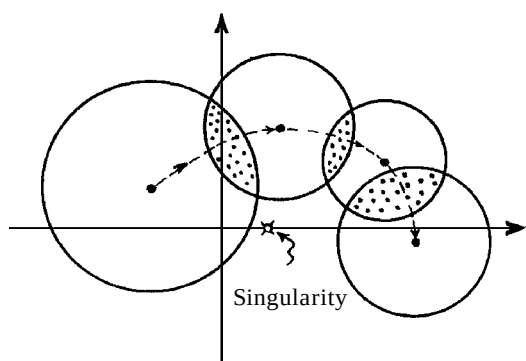
Fig. 7.6 A holomorphic function can be analytically continued, using a succession of power series expressions about a sequence of points. This proceeds uniquely along the connecting path, assuming successive circles of convergence overlap.
