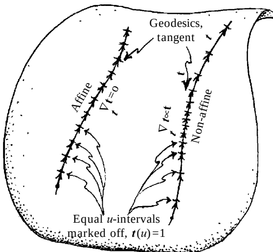
Fig. 14.8 For any (suitably smooth) parameter u defined along a curve \gamma , a field of tangent vectors \mathbf{t} to \gamma is naturally associated with u so that, along \gamma , \mathbf{t} stands for d/du (equivalently \mathbf{t}(u) = 1 , or t^a \nabla_a u = 1 ). If \gamma is a geodesic, u is called an affine parameter if \mathbf{t} is parallel-transported along \gamma , so \nabla_{\mathbf{t}}\mathbf{t} = 0 rather than just \nabla_{\mathbf{t}}\mathbf{t} \propto \mathbf{t} . An affine parameter is ‘evenly spaced’ along \gamma , according to \nabla .
