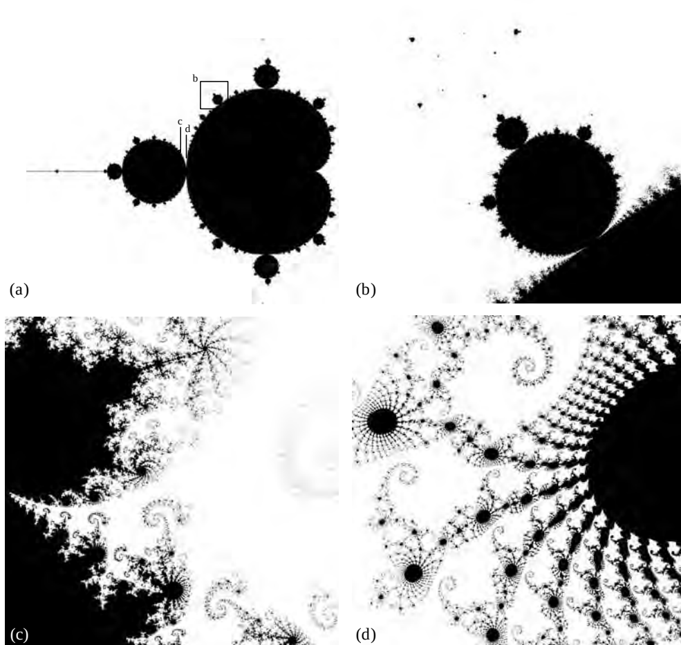
Fig. 1.2 (a) The Mandelbrot set. (b), (c), and (d) Some details, illustrating blow-ups of those regions correspondingly marked in Fig. 1.2a, magnified by respective linear factors 11.6, 168.9, and 1042.
