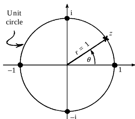
Fig. 5.8 The unit circle, consisting of unit-modulus complex numbers. The Cotes–Euler formula gives these as e^{i\theta} = \cos \theta + i \sin \theta for real \theta .
