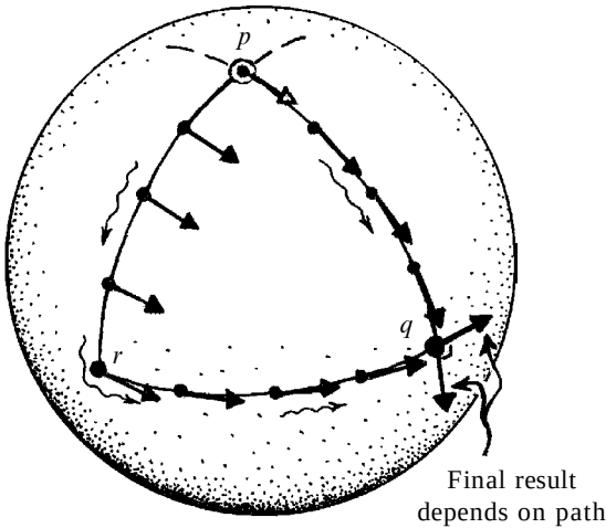
Fig. 14.4 Path dependence of parallel transport. This is illustrated using two distinct paths from p to q , one of which is a direct great-circle route, the other consisting of a pair of great-circle arcs jointed at an intermediate point r . Parallel transport along these two paths gives results at q differing by a right-angle rotation.
