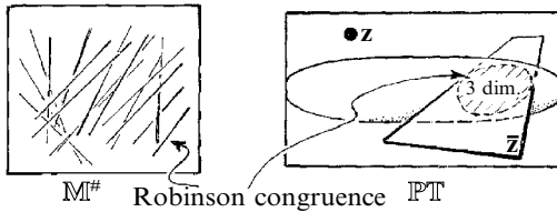
Fig. 33.14 We can obtain a ‘real’ picture of a non-null twistor Z^\alpha by first passing to its complex conjugate \bar{Z}_\alpha , thus defining a complex projective plane in \mathbb{P}^7\mathbb{T} . This plane is fixed by its intersection with \mathbb{P}^N , which is a 3-real-dimensional locus. This locus defines a 3-parameter family of light rays in \mathbb{M}^\# called a Robinson congruence.
