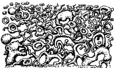
Fig. 29.6 What is the nature of spacetime at the Planck scale of 10^{-33}\text{ cm} or 10^{-43}\text{ s} ? It has been argued that quantum fluctuations in the gravitational field may result in a seething mess of ‘foam’ with multiple topology changes, and where possibly detailed quantum phase relations may actually get lost at this level.
