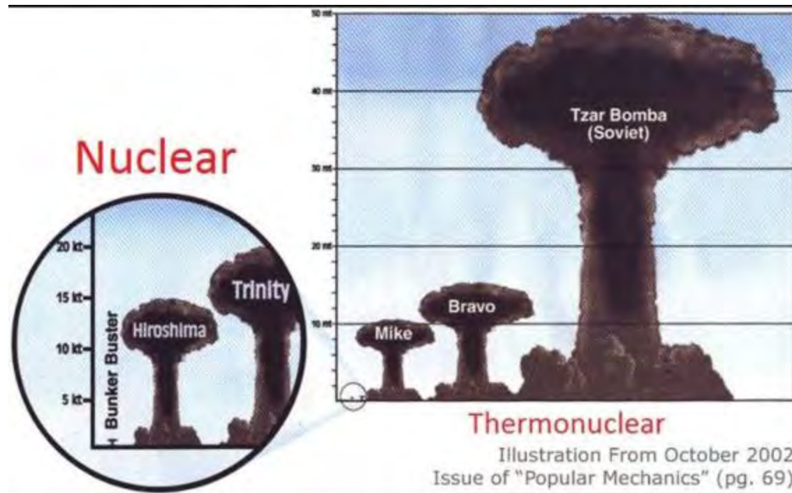
Figure 5. Size comparison of nuclear detonations
