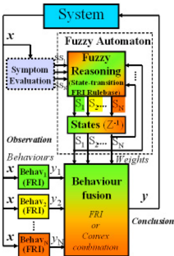
Fig. 11 The suggested FRI behaviour-based structure.
